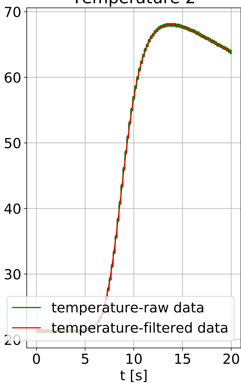
Temperature 2
