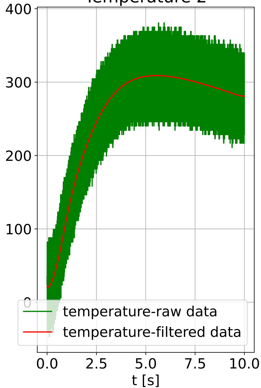
Temperature 2
