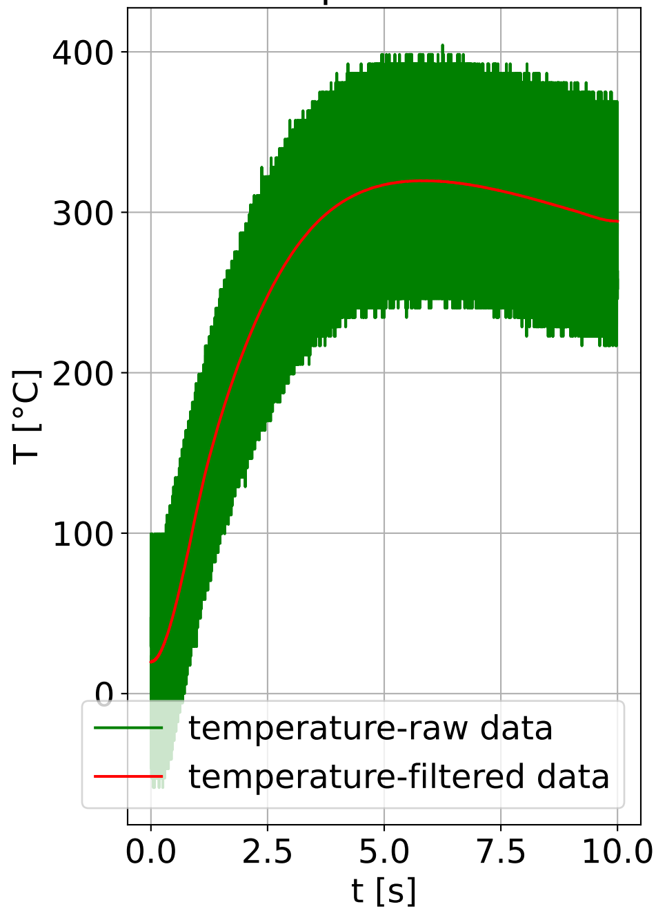
Temperature 1
