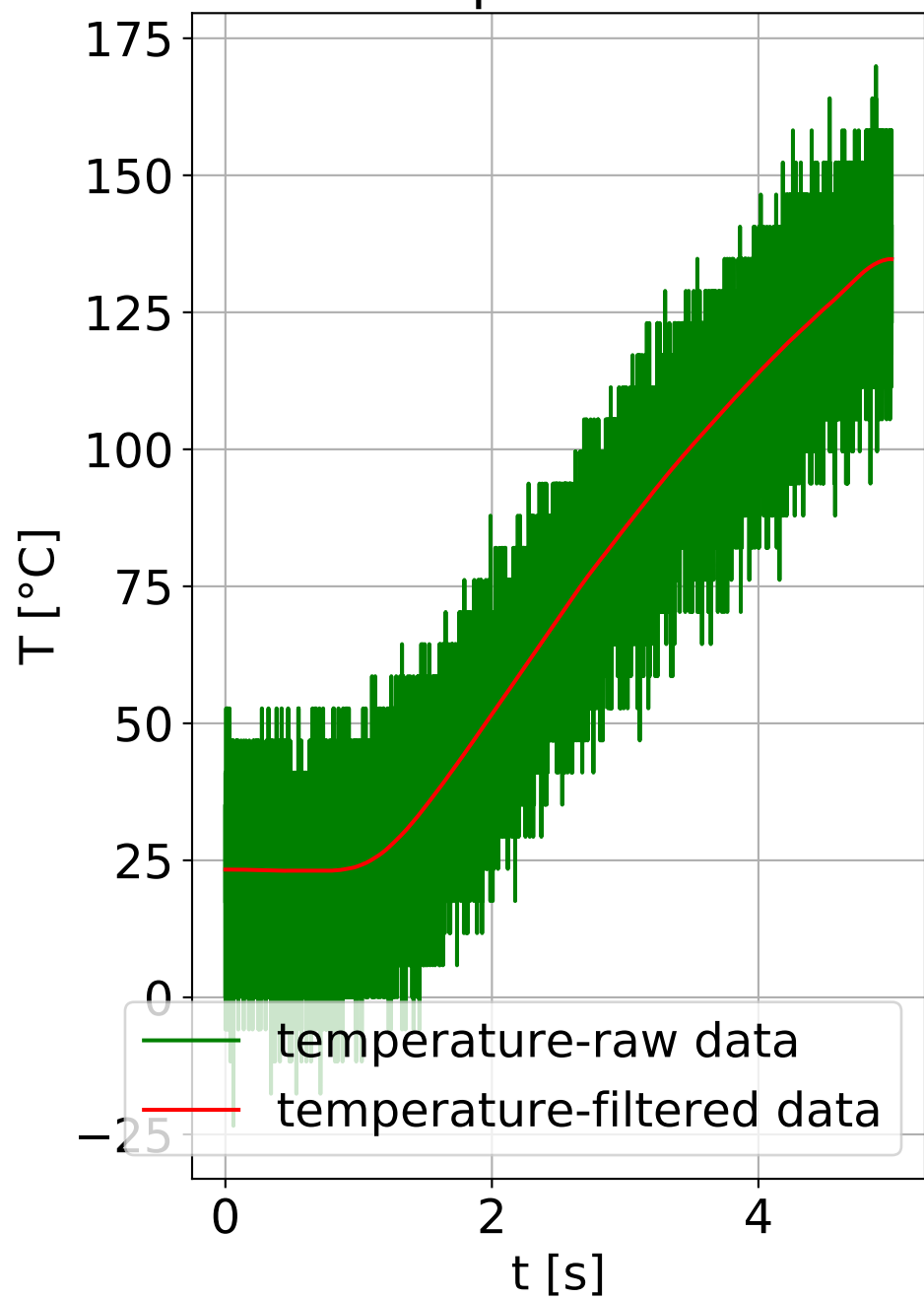
Temperature 1
